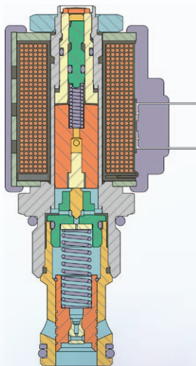
Cartridge Valve Cut Away
